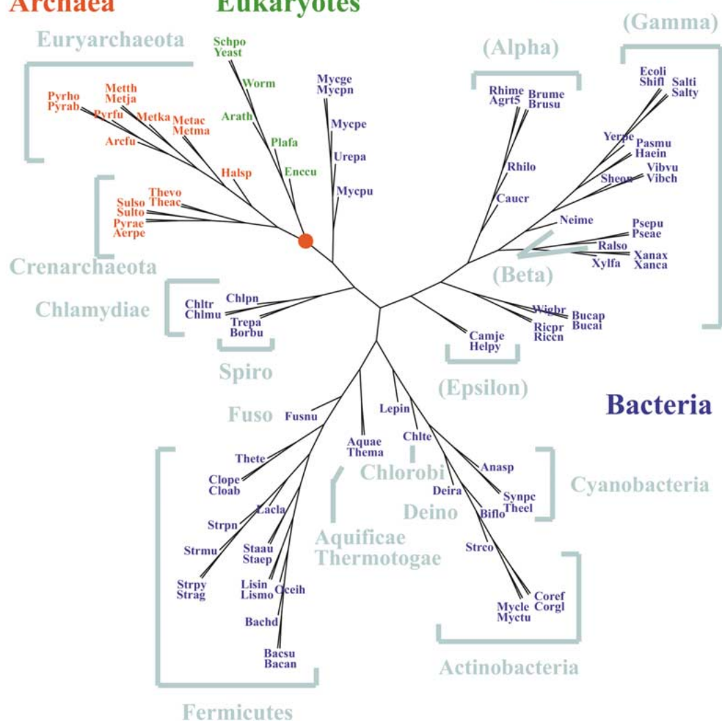
Fig. 1. A K = 6 phylogenetic tree for 109 organisms. Different strains within the same species were represented by one strain so there are 93 species shown in the tree. The red dot denotes the trifurcation point of the three domains. Archaea, Bacteria, and Eukarya are indicated by red , blue , and green , respectively. All 13
