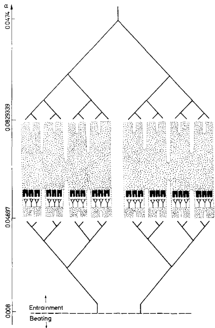
Fig. 3. Hierarchy of period-doubling bifurcation sequences (schematic, not to scale). Only one secondary sequence embedded in a 8I band is shown.
