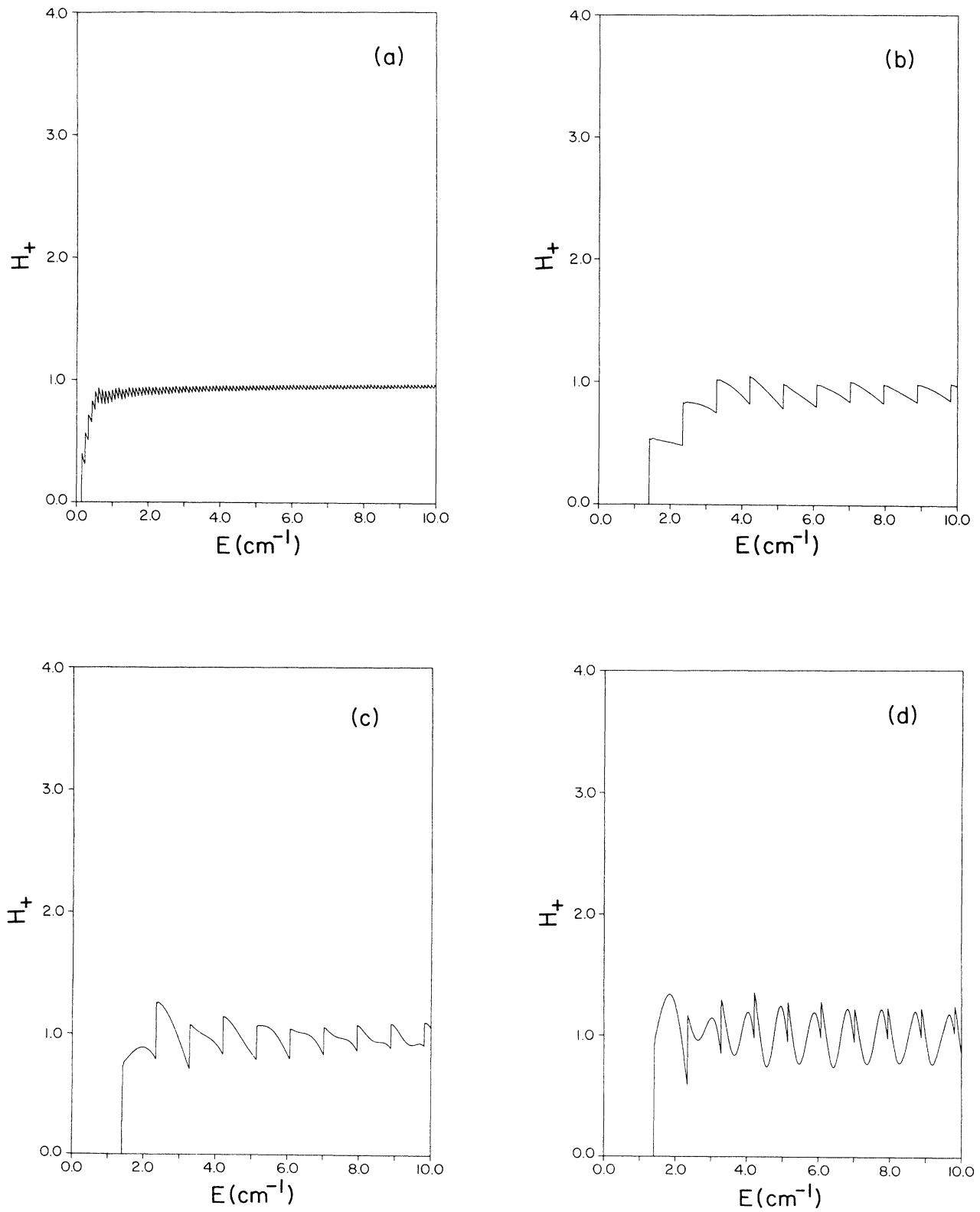
FIG. 2. The factor H_+(E, F, B) defined in Eq. (15b) plotted as a function of E for the electric and magnetic fields listed in Table I. H_+ multiplied by the smooth zero-field cross section \sigma_0(E) in Eq. (15) gives the photodetachment cross section of \text{H}^- in parallel electric and magnetic fields with photons circularly polarized. Note H_+ fluctuates around a mean value of unity.
