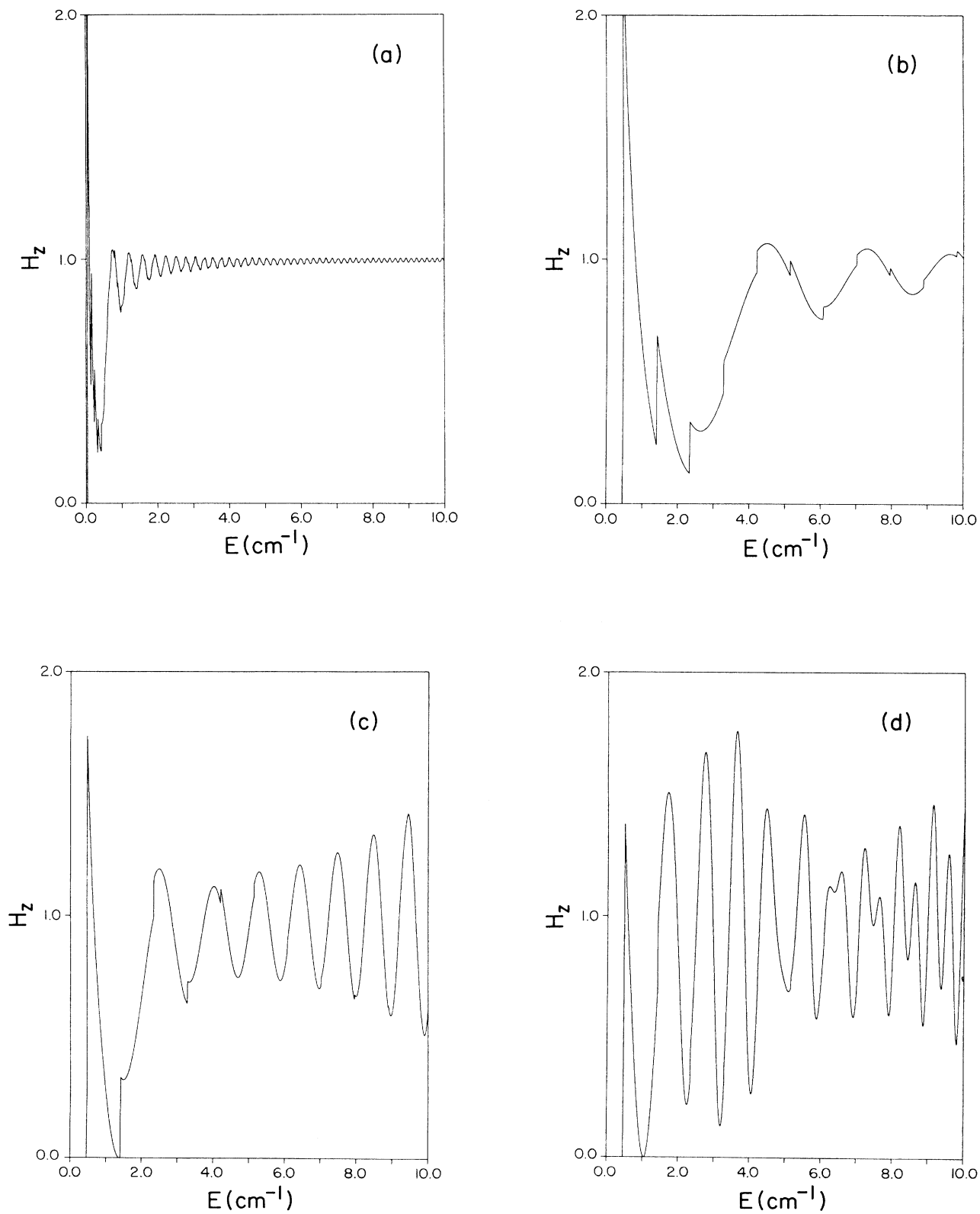
FIG. 1. The factor H_z(E, F, B) defined in Eq. (13b) plotted as a function of E for the electric and magnetic fields listed in Table I. H_z multiplied by the smooth zero-field cross section \sigma_0(E) in Eq. (14) gives the photodetachment cross section of \text{H}^- in parallel electric and magnetic fields with photons linearly polarized along the fields. Note H_z fluctuates around a mean value of unity.
